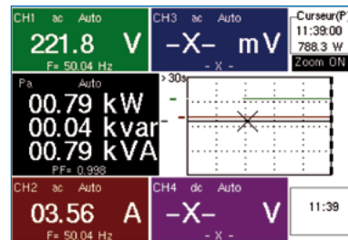
Display of apparent, active and reactive power and the PF
