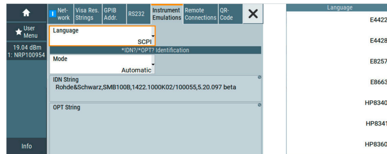
The emulation mode can be set in the remote setup menu of the R&S®SMB100B.
