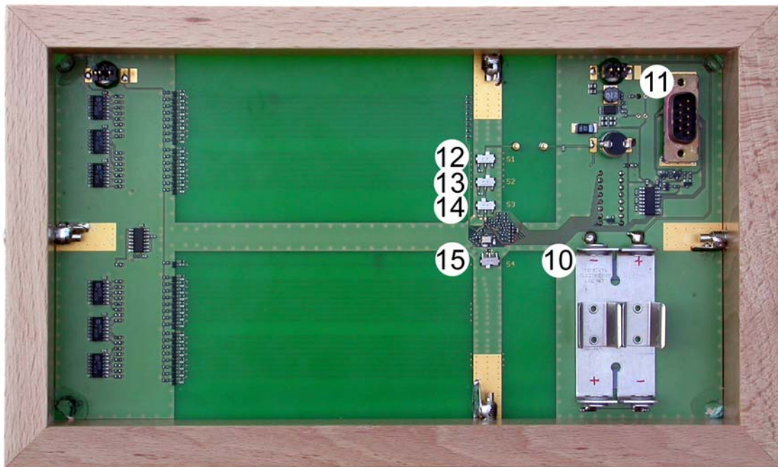
Figure 3.2: OIVM 251 rear
