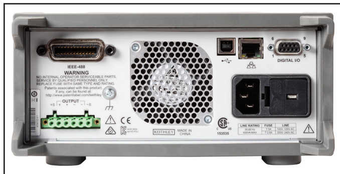
Figure 7. 2281S rear panel.
