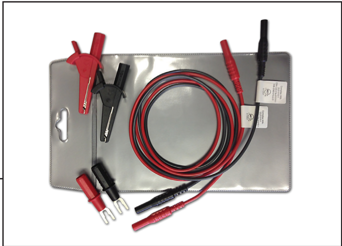
Model 2280-TEST-LEAD: Power Supply Test Lead Kit, 1000V, 20A Rating: Contains 122cm (4ft) of cable, spade lug adapters, and alligator clips
